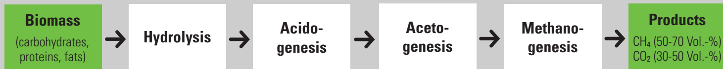
Cascade laboratory/methanisation plant
