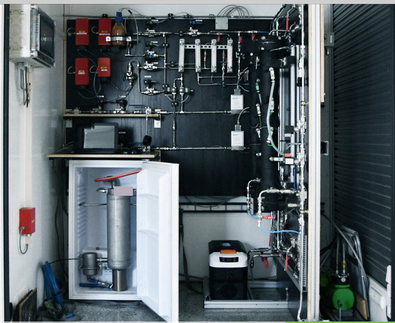
Mobile test stand
